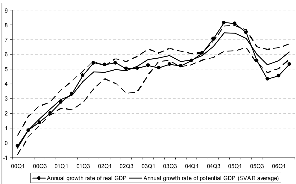
Figure 5. Annual growth rates of potential GDP - SVAR
