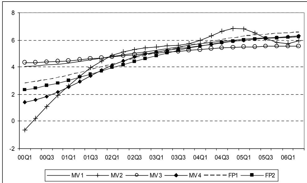
Figure 4. Annual growth rates of potential GDP – multivariate filters (MV) and production function (PF)
