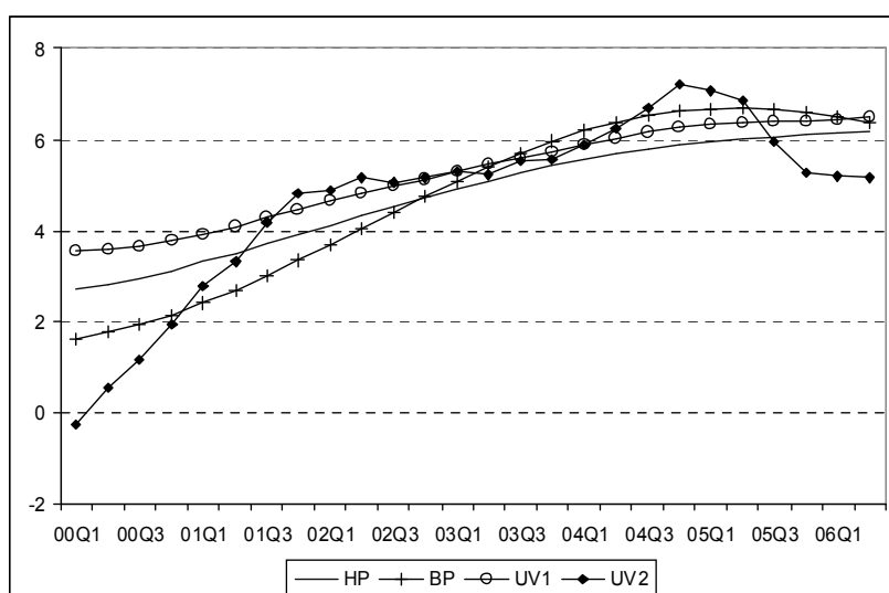
Figure 2: Annual growth rates of potential GDP – univariate filters
