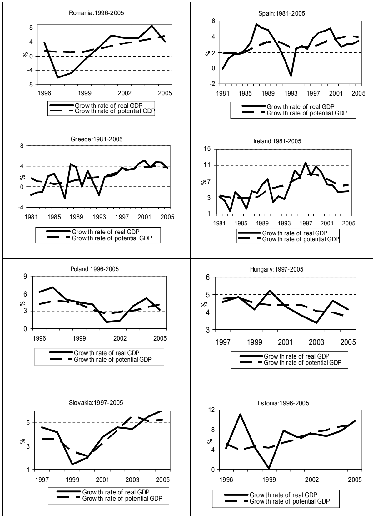
Figure 1. Growth rates of actual and potential real GDP for eight countries
