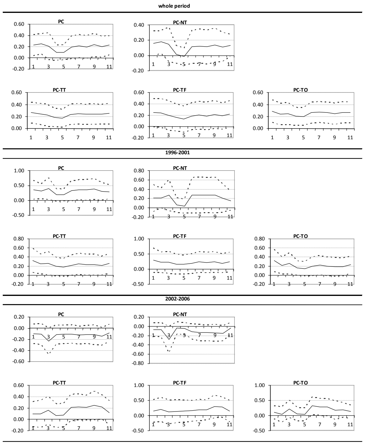
Figure 3: Accumulated Impulse Response after 6 Periods; m-o-m Data
